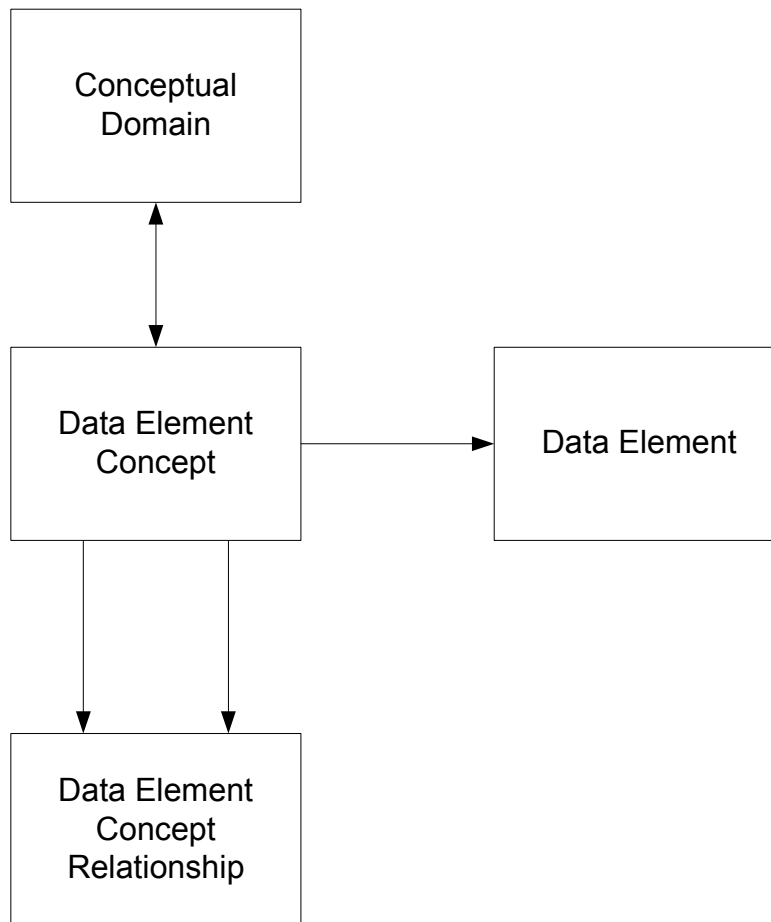
Figure 4. 11179 Meta Model Data Element Concept Region
