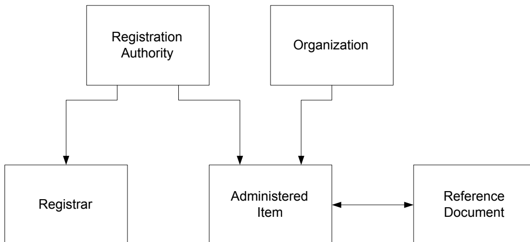
Figure 2.11179 Meta Model Administration and Identification Region
