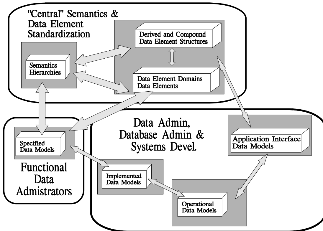
Figure 8. Integration of semantics and data element model with other essential to enterprise-wide data standardization data metadata models.
