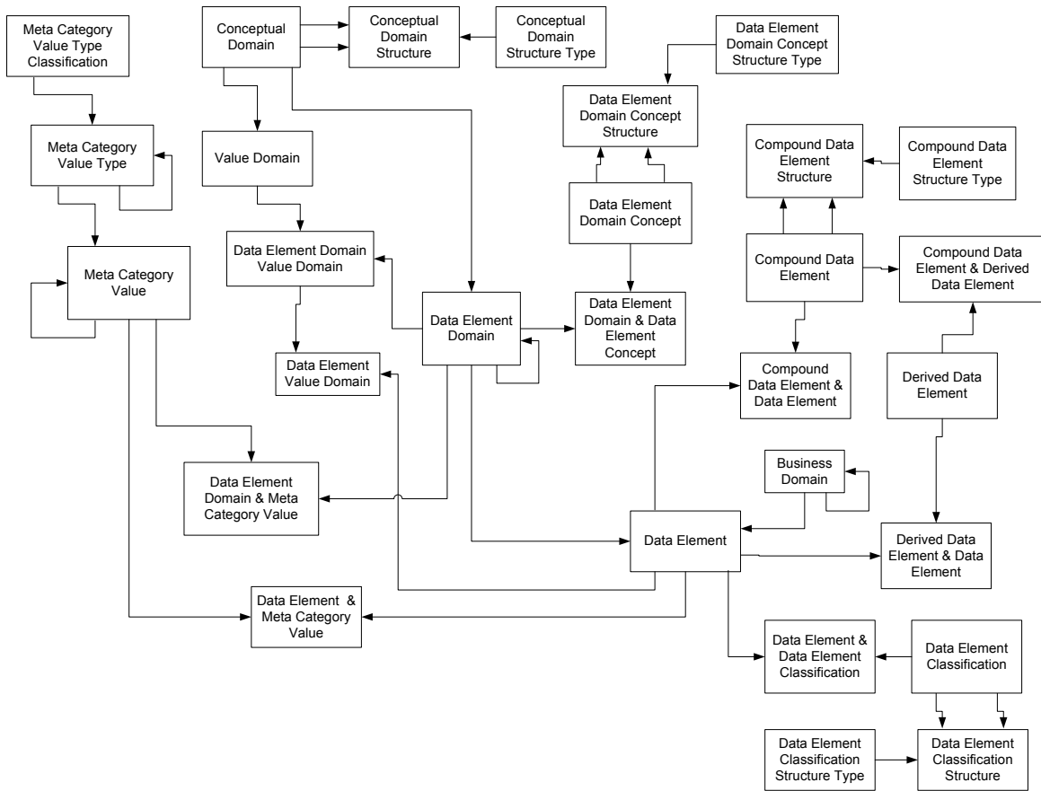
Figure 7. Transformed “relational” data element model for 11179.
